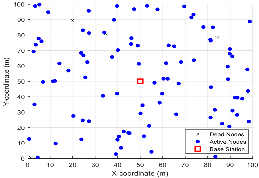
Figure 3. Distribution of nodes (active and dead nodes) along with the base station during simulation.
