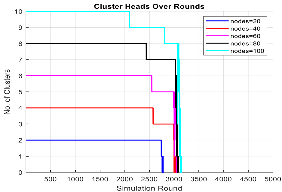
Figure 4. Typical graph for the number of Clusters over Rounds for different no. of Nodes
