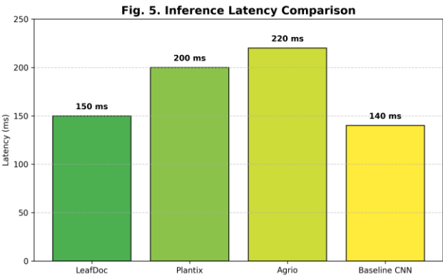
Fig 5 – Inference Latency Comparison Across Models
