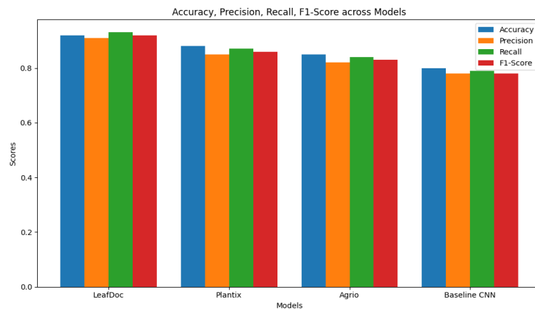
Fig 7. – Bar Chart: Accuracy, Precision, Recall, F1-score across Models
