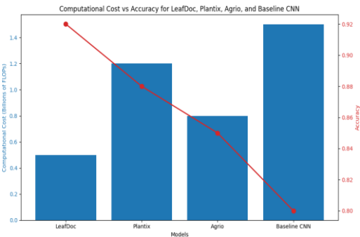
Fig.6. Computational Cost Vs Accuracy
