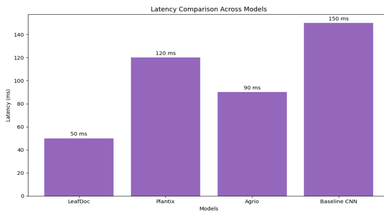
Fig 8– Latency Comparison Across Models
