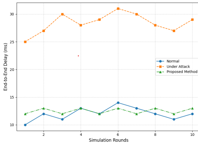
Figure 11. Delay Analysis
