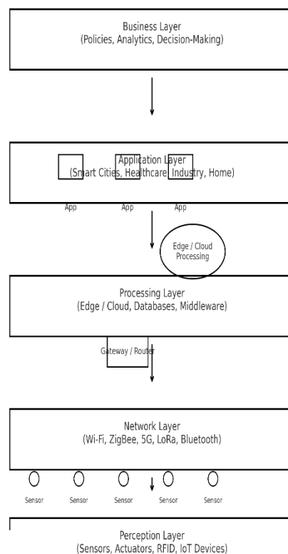
Figure 1. Schematic Representation of IoT
