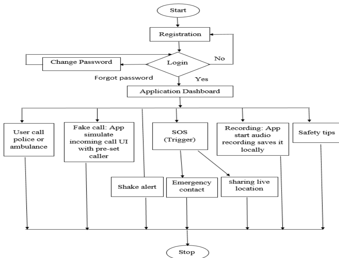
Figure 1. Proposed Methodology for Women's Safety Analytics
