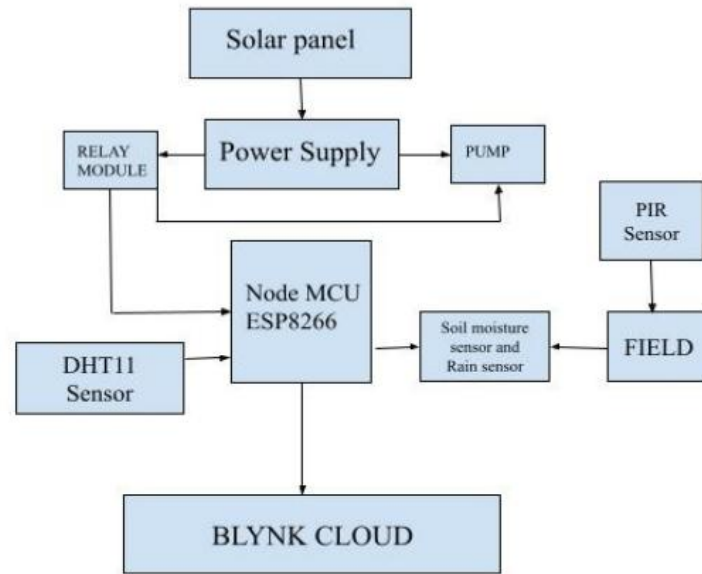
Fig 1: IoT-Based Smart Irrigation System Block Diagram
