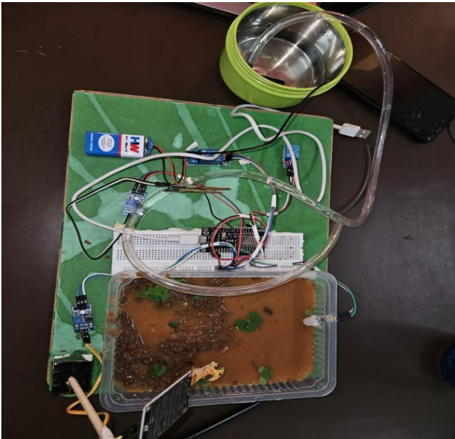
Fig 2: Implementation Scenario of Smart Irrigation System
