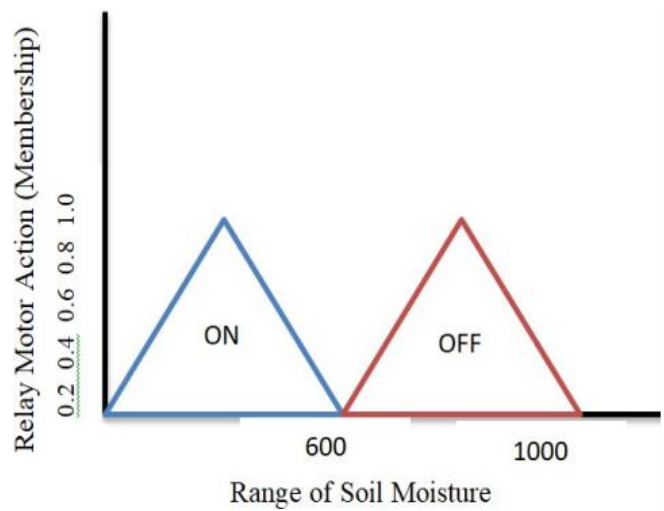
Fig 4: Fuzzy Logic Concept From Soil Moisture and Relay Motor Action
