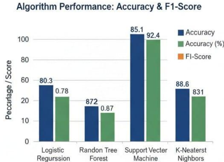
Figure 2: Algorithm performance
